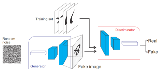
Figure 1: GAN structure
