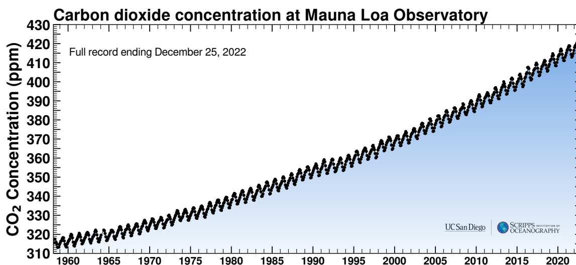
Figure 2.1: Mauna Loa observatory CO 2 measurement (R. F. Keeling and C. D. Keeling, 2017)
