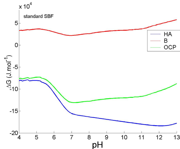
Figure 1: Gibbs free energy variations: simulated results.
