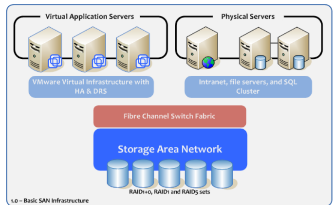
Figure 1. SAN Architecture
