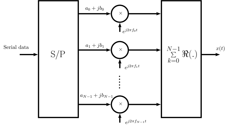
Figure 2.1: Block diagram of MCM transmission (Yang, 2009).
