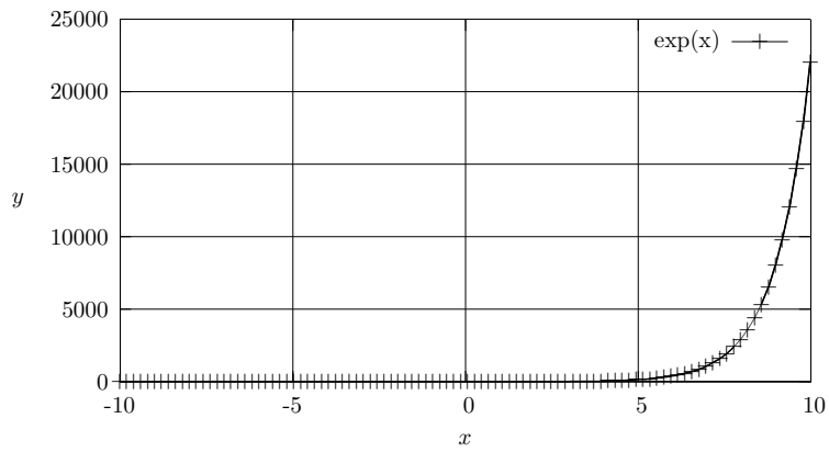
gnuplottex test e^x
